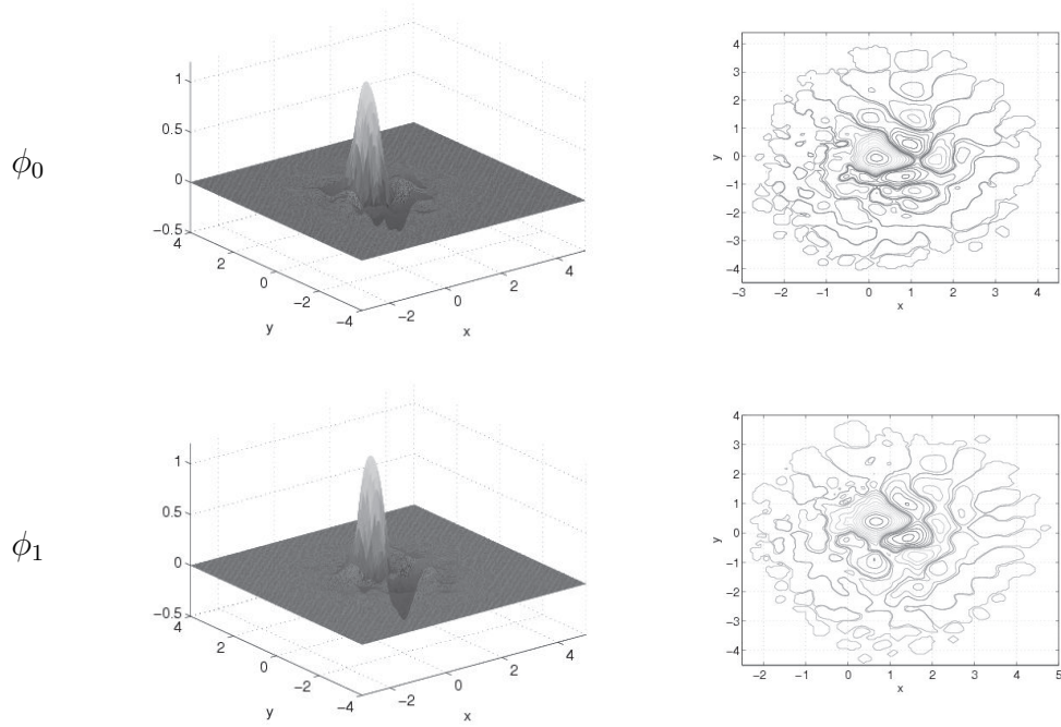
Figure 4: Component functions of \Phi_5^q
