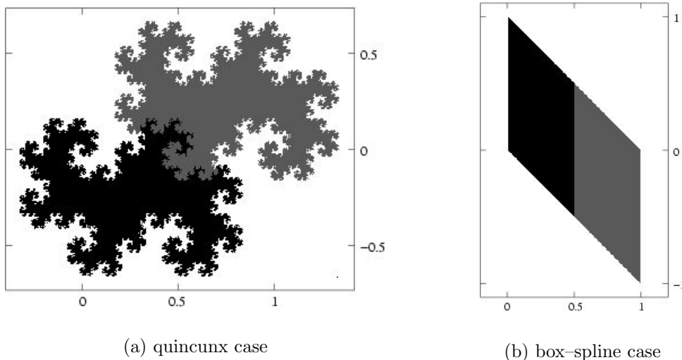
Figure 1: (Multi-) tiles corresponding to \Phi_0
