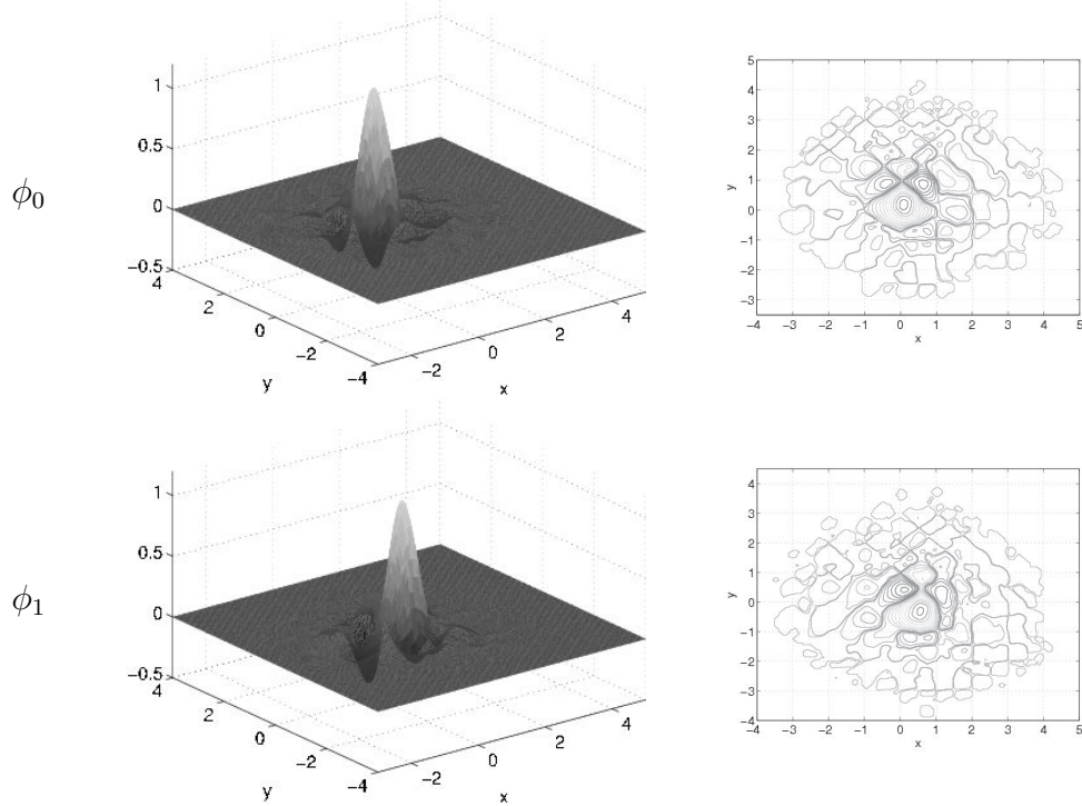
Figure 5: Component functions of \Phi_5^b
