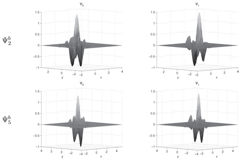
Figure 7: Multiwavelets corresponding to \Phi^b
