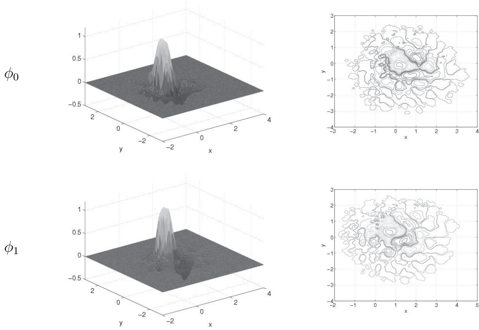
Figure 2: Component functions of \Phi_2^q
