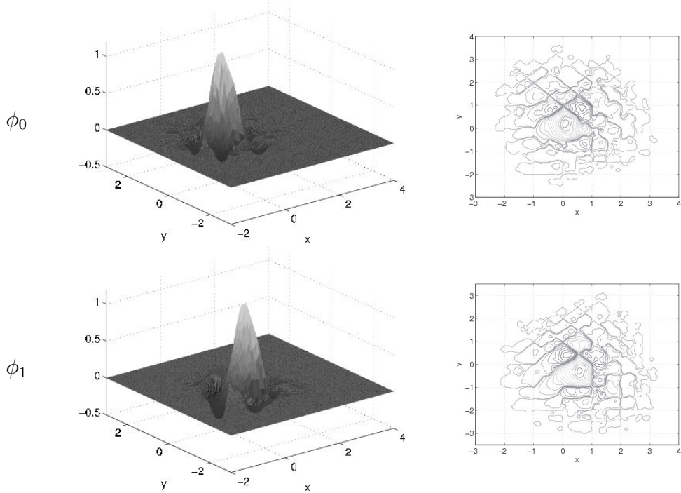
Figure 3: Component functions of \Phi_2^b
