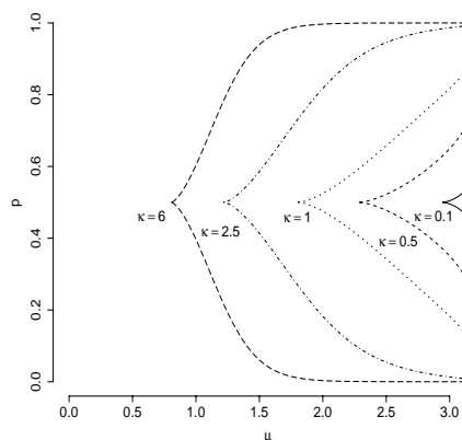
Figure 2: Regions of bimodality of the von Mises distribution, where \mu = \mu_2 - \mu_1 and \kappa_1 = \kappa_2 = \kappa .
