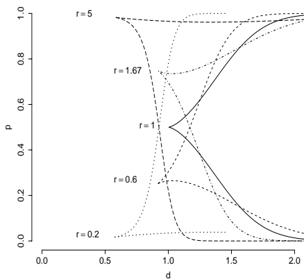
Figure 1: Regions of bimodality of the normal distribution, where d = (\mu_2 - \mu_1)/(2\sqrt{\sigma_1\sigma_2}) and r = \sigma_1/\sigma_2 .
