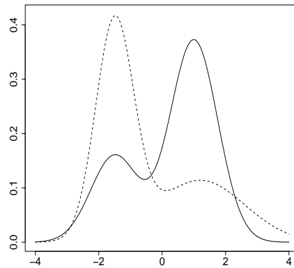
Figure 4: Densities of normal mixtures f_2(x) = f(x, 0.3, -1.5, 1, 0.75, 0.75) (solid line) and f_3(x) = f(x, 0.6, -1.5, 1.4, 0.6, 1.4) (dashed line)
