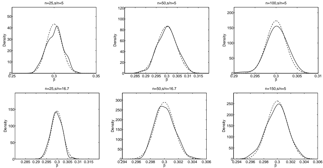
Figure 5: Simulated (solid curve) and asymptotic (dashed curve) distributions of \hat{\beta}_{\Delta, N} for f_1 . The variance of the asymptotic distributions is given as \frac{8\sigma^2\Delta^2}{M_N''(\beta^*)} (cf. Theorem 3). The parameter N was chosen as 7, 8, 12 (first row, left to right), and 8, 12, 12 (second row, left to right).
